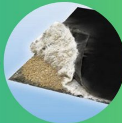
Laminated GCL
